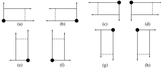
Fig. 5. Local Refinement Scheme
